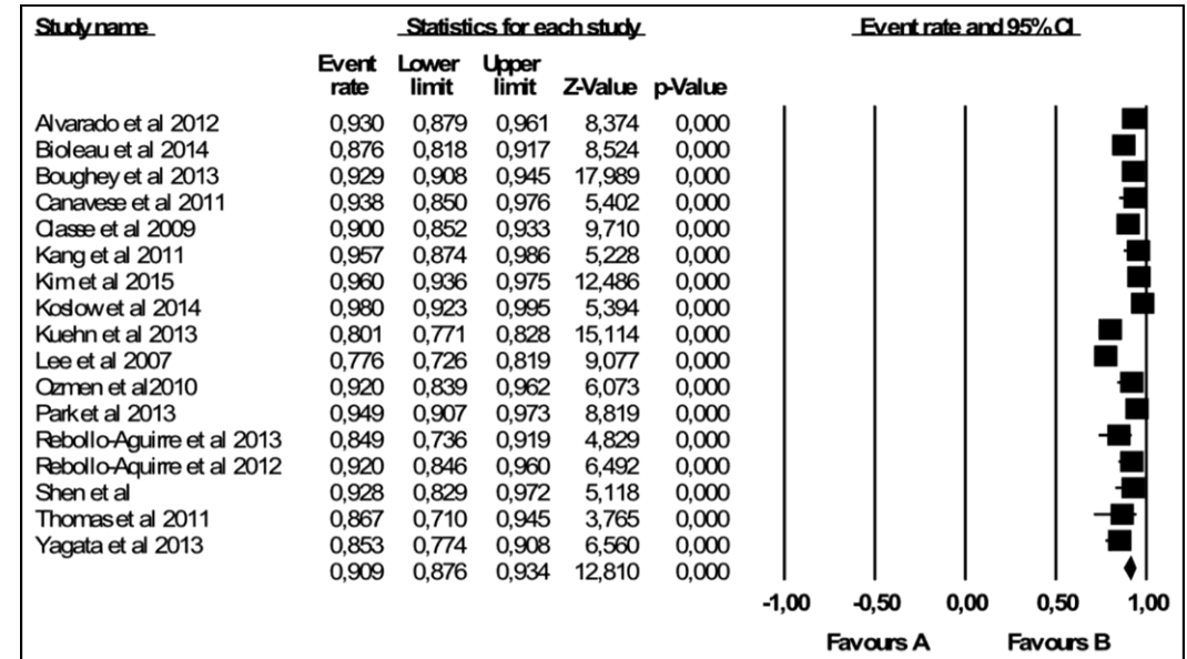
Figure 4 Forest plot showing event rate defined as IR. Seventeen studies were included. The pooled estimate was found to be 90.9% (95% CI 87.6% to 93.4%).
