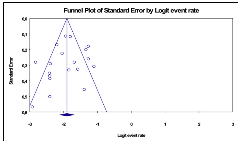
Figure 3 Meta-analysis of FNR: a funnel plot to examine for evidence of publication bias. According to the funnel plot of logit FNR vs standard, there seems to be no publication bias with respect to the list of 19 studies reporting FNR.
