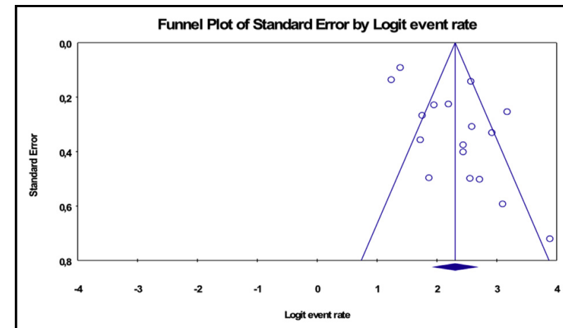
Figure 5 Meta-analysis of IR: a funnel plot of the included studies, estimated based on random effects analysis is relatively balanced, favoring the conclusion that there is no publication bias.
