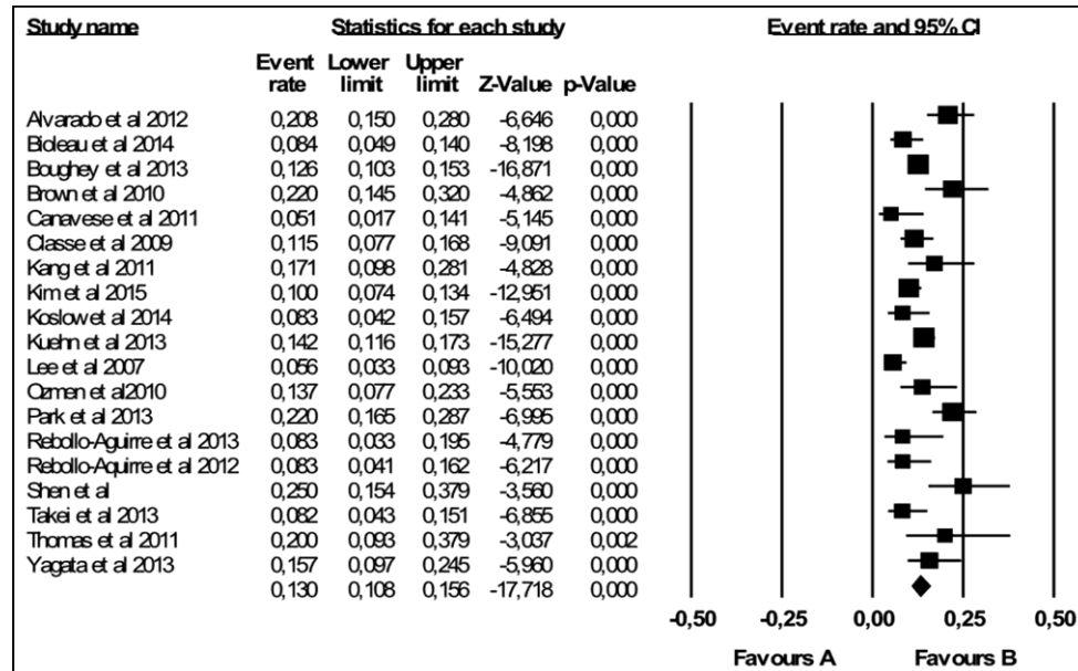
Figure 2 Forest plot showing event rate defined as FNR. Nineteen studies were included. The pooled estimate was found to be 13% (95% CI 10.8% to 15.6%).
